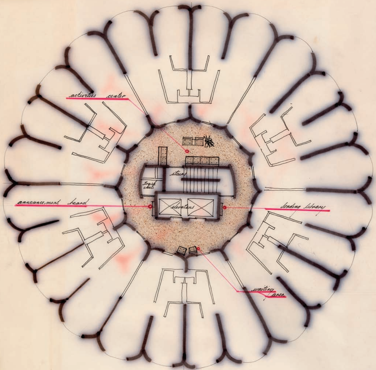
social center plan (each floor)
